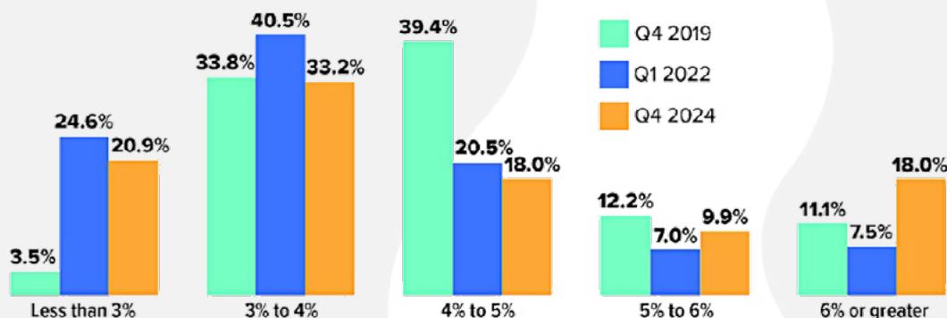
Share of outstanding mortgages by interest rate
